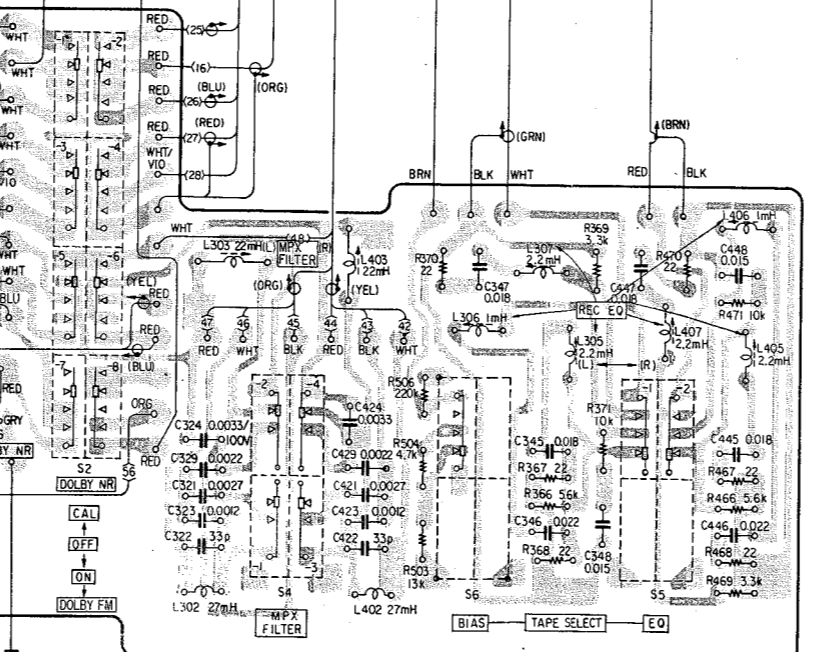
[ SWITCH BOARD ]
