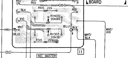
[ MASTER CONTROL BOARD ]
