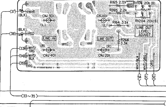
[ JACK BOARD ]
